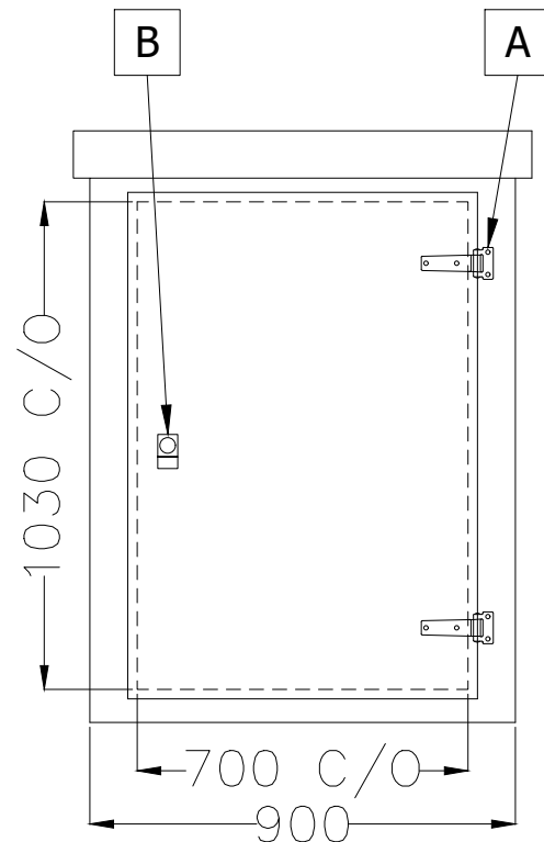
EXTERNAL VIEW ON FRONT WALL
