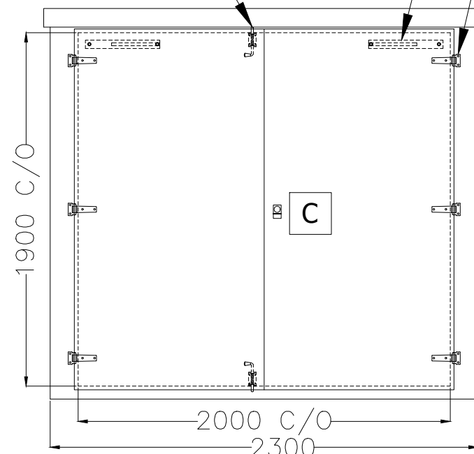
EXTERNAL VIEW ON FRONT WALL
