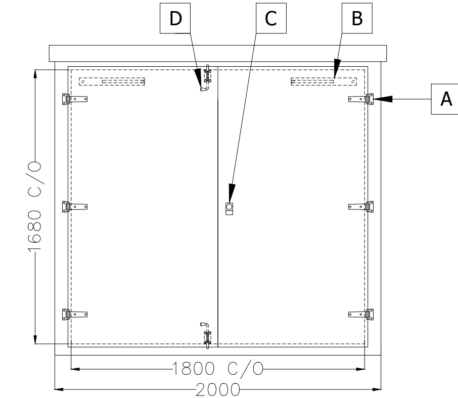
EXTERNAL VIEW ON FRONT WALL
