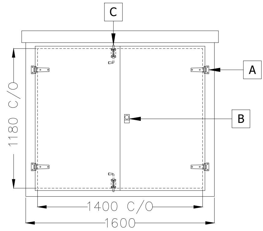
EXTERNAL VIEW ON FRONT WALL
