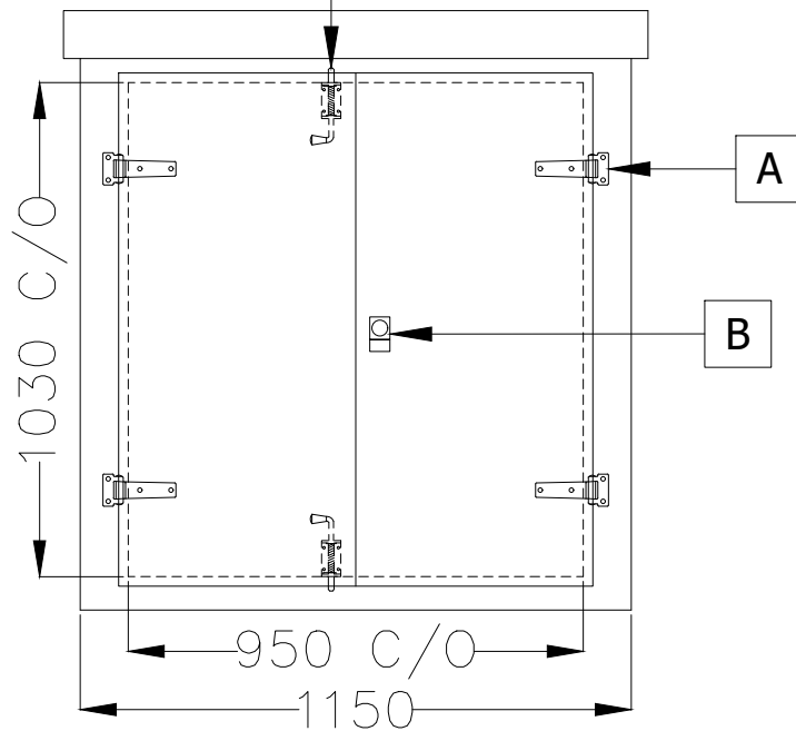
EXTERNAL VIEW ON FRONT WALL
